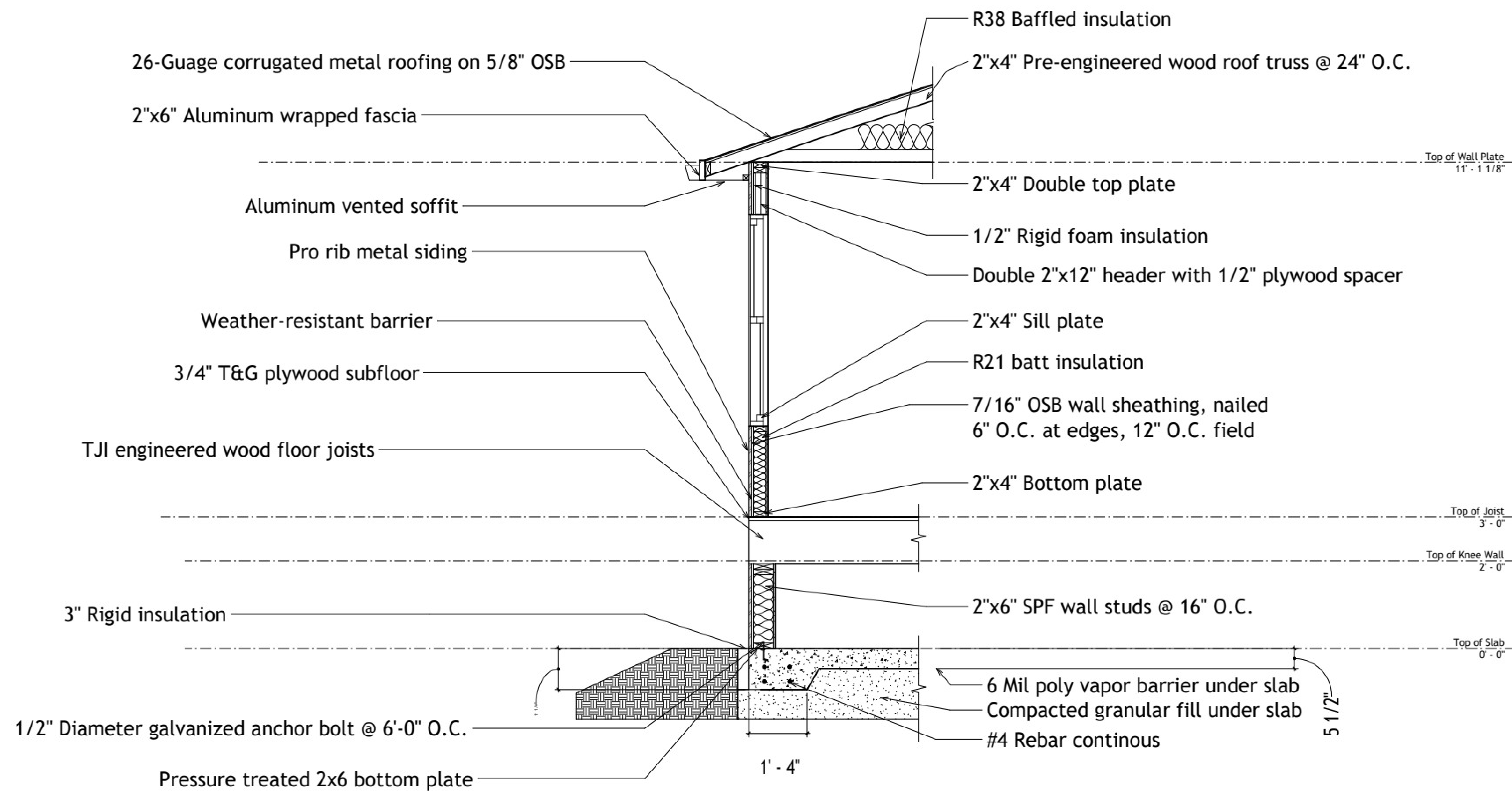
① Exterior Wall Detail Section 3/4" = 1'-0"
