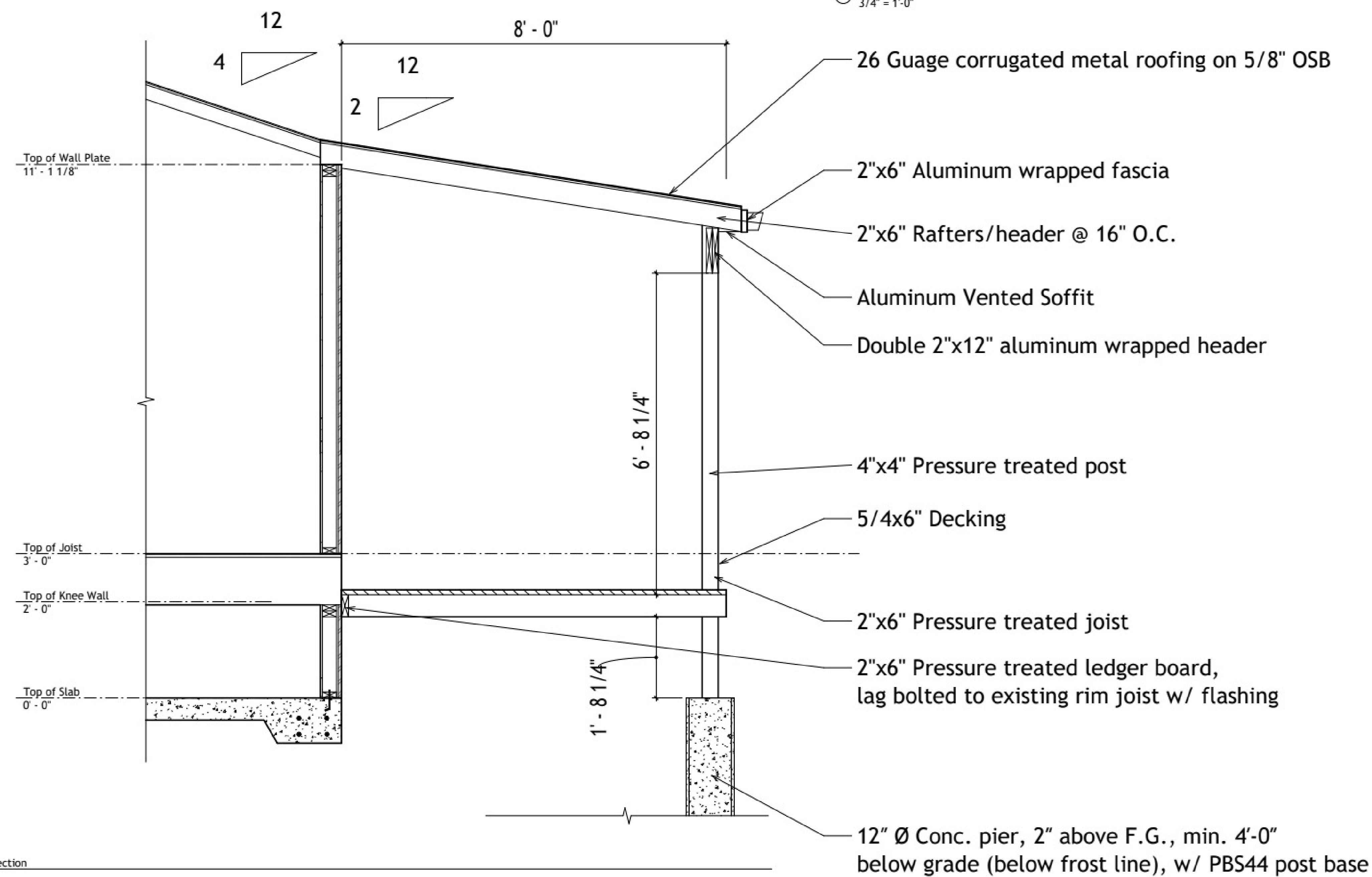
① Exterior Wall Detail Section 3/4" = 1'-0"
