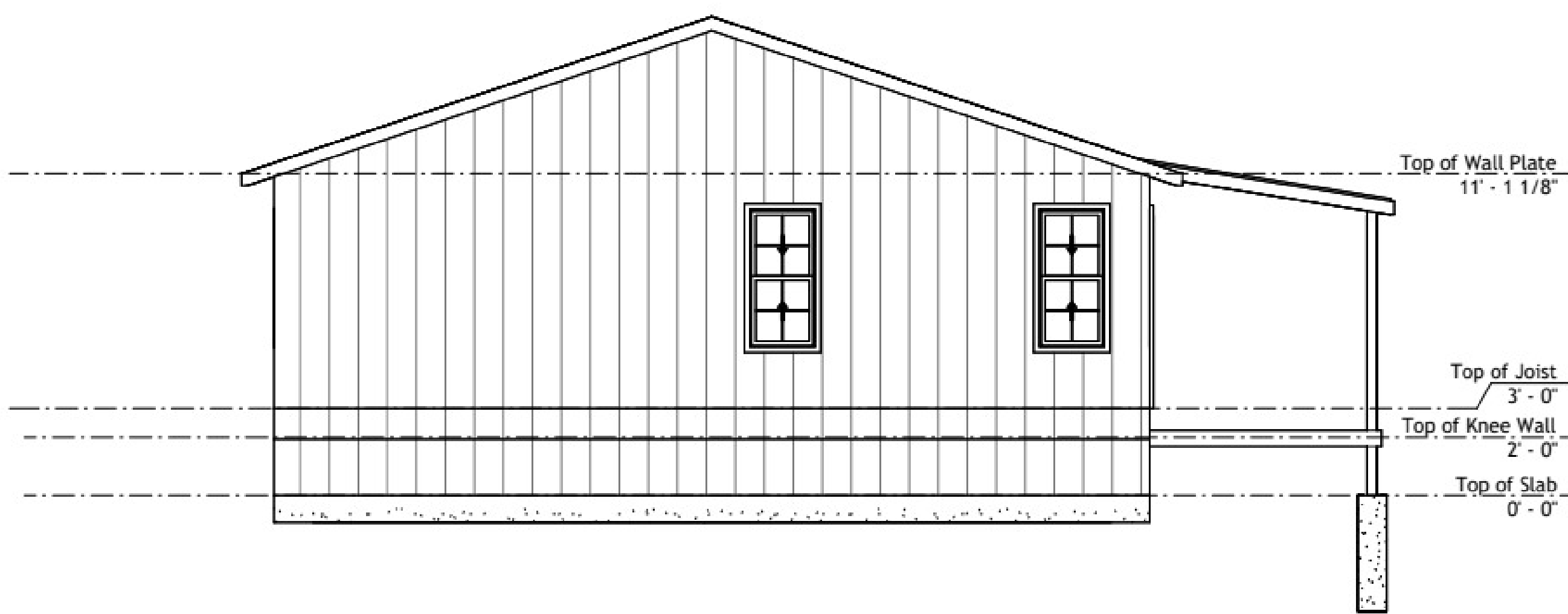
④ West Architectural Building Elevation 1/4" = 1'-0"
