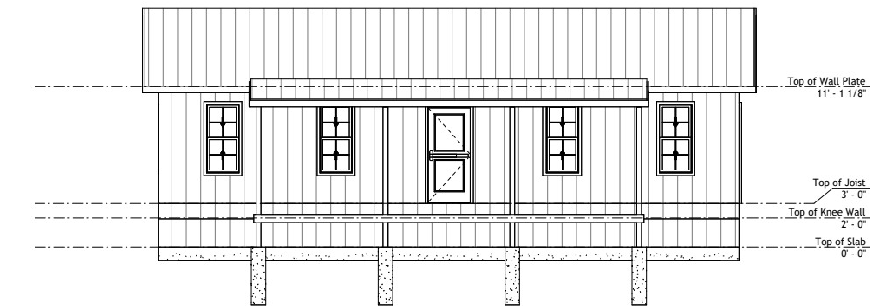
② South Architectural Building Elevation 1/4" = 1'-0"
