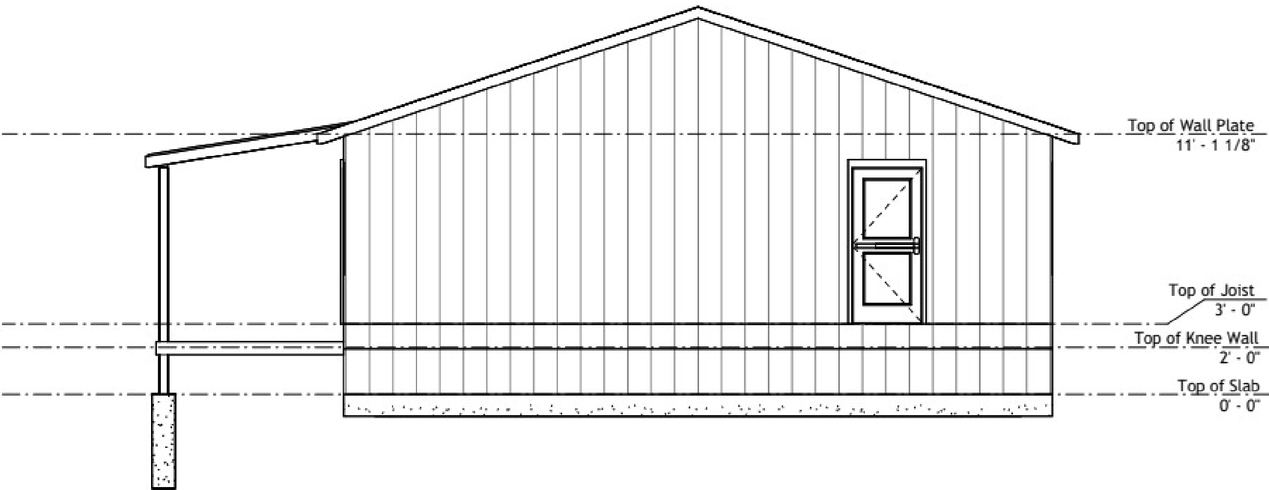
③ East Architectural Building Elevation 1/4" = 1'-0"
