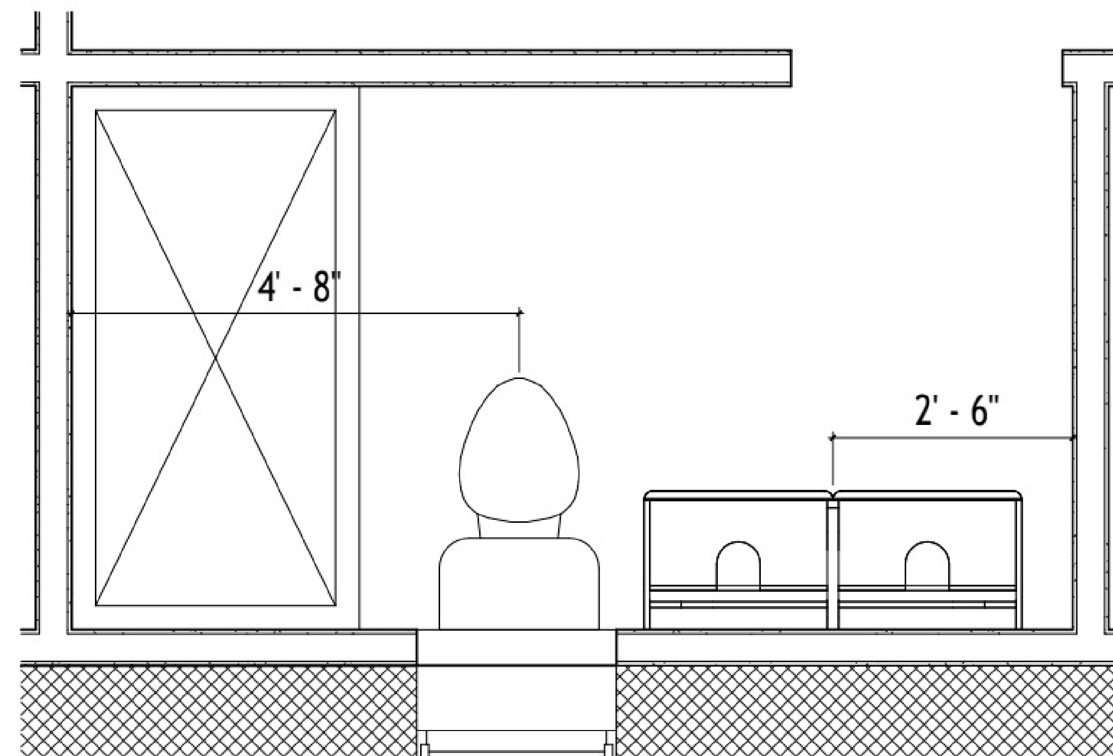
① Second Floor Master Bath 1" = 1'-0"
