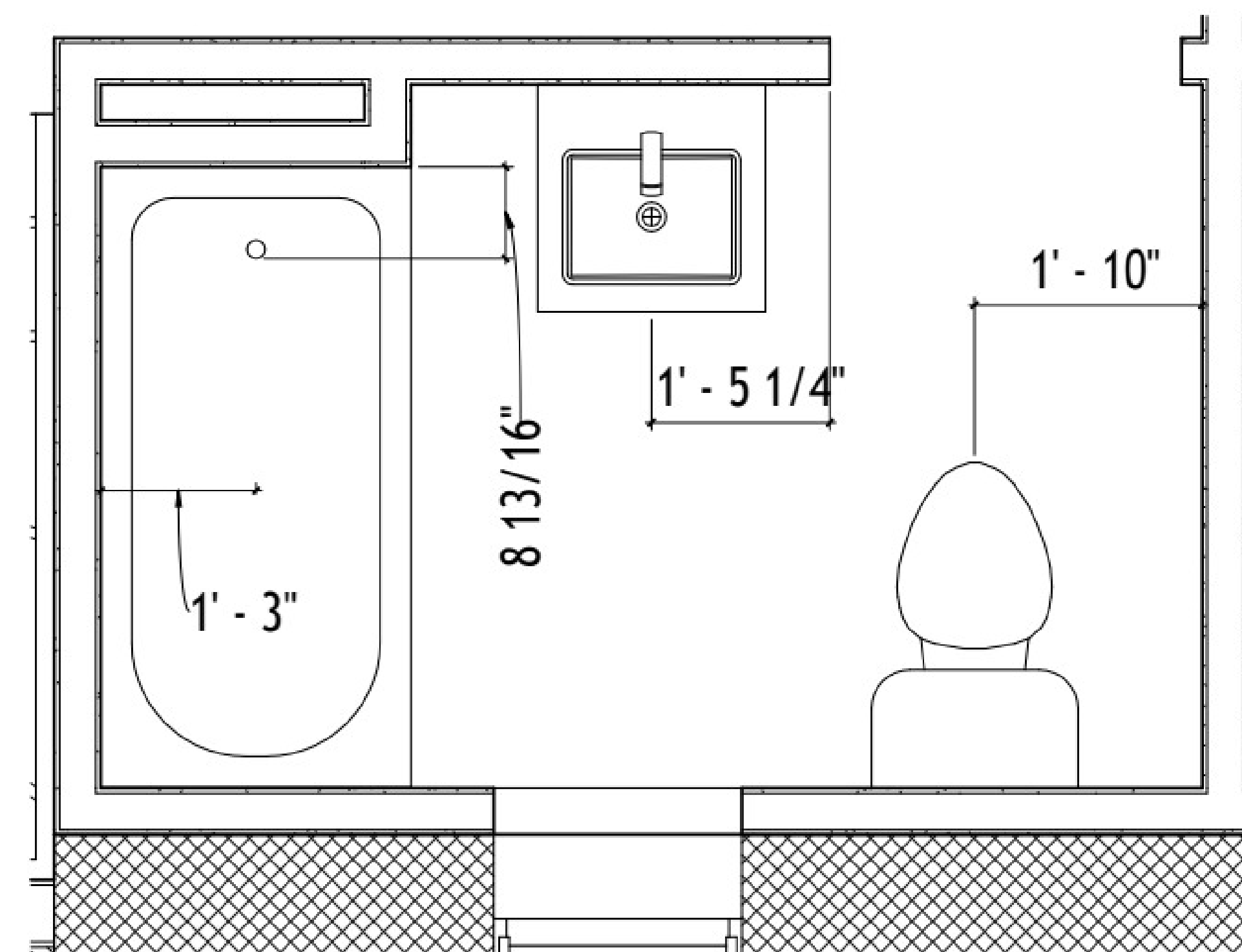
② Second Floor Bath 1" = 1'-0"
