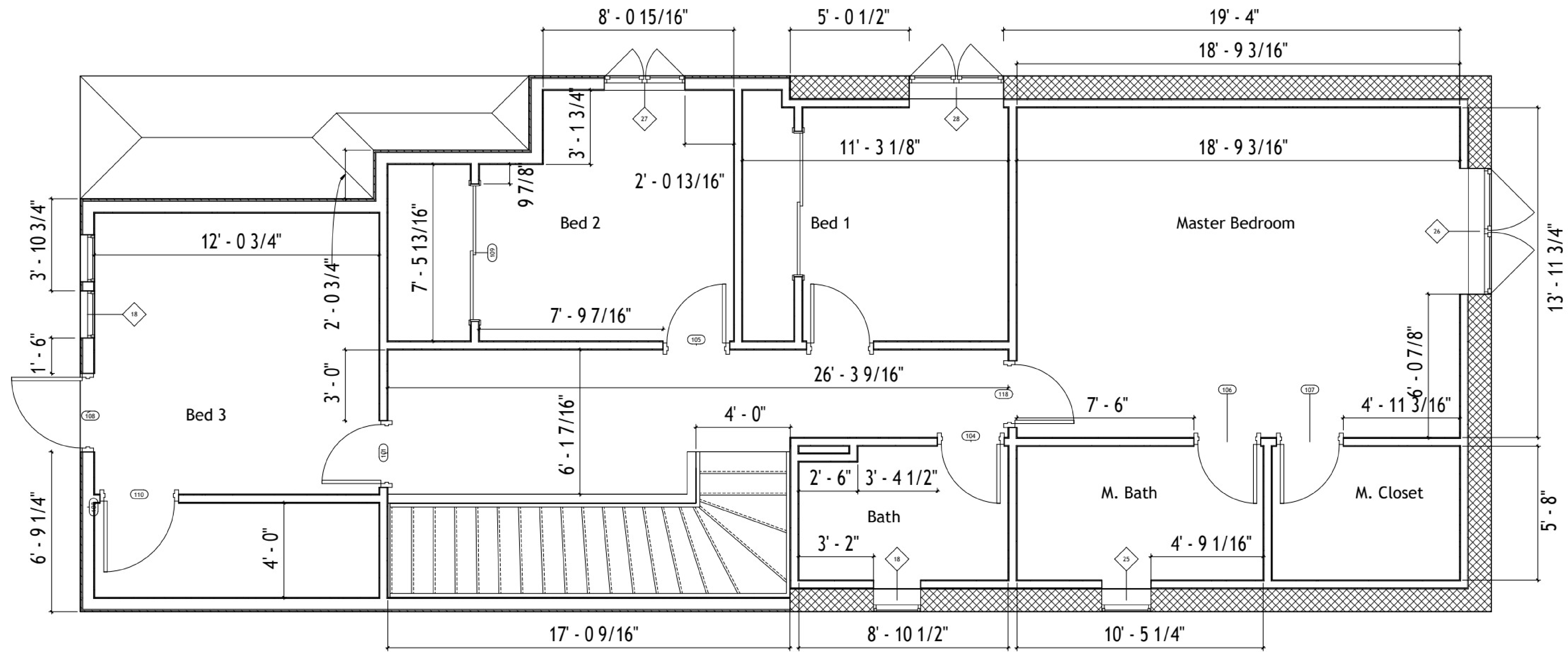
① Second Floor Architectural Plan 1/2" = 1'-0"
